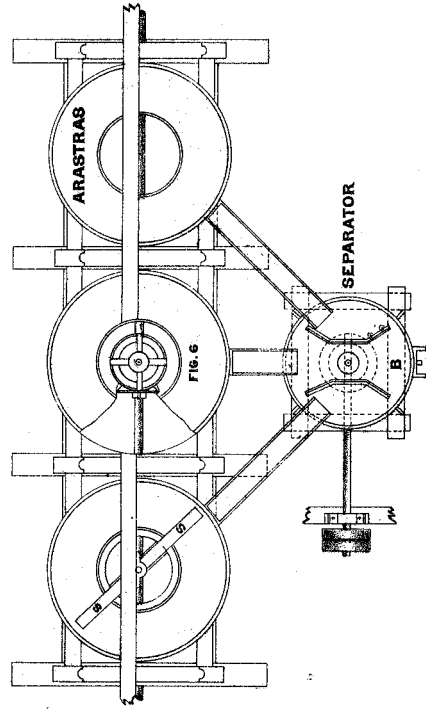
PLAN OF ARASTRAS AND SEPARATOR
