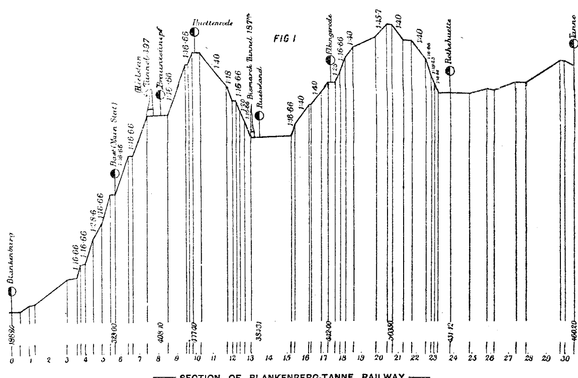
— SECTION OF BLANKENBERG-TANNE RAILWAY. —
