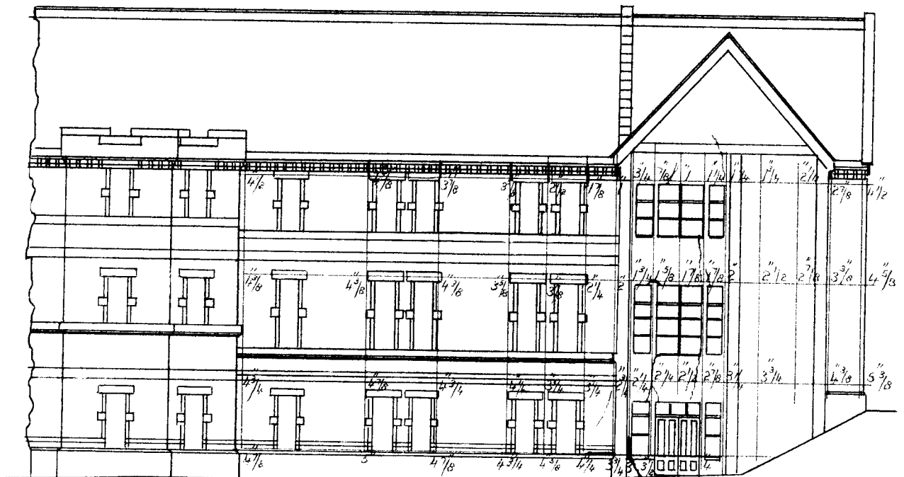
NORTH ELEVATION OF NORTH WING
