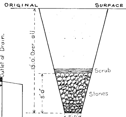
DRAIN N.O.1 Cross Section Scale 5 Ft.=1 in.
