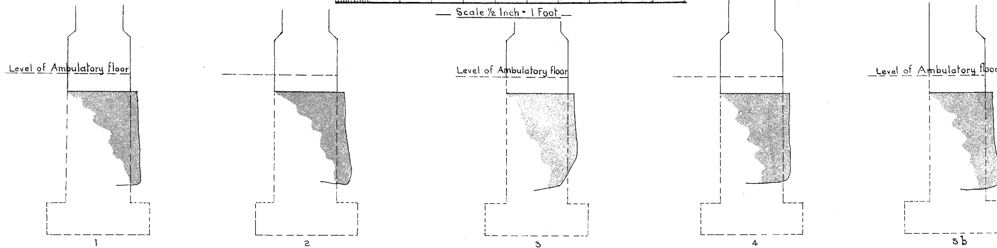
Foundations of Ambulatory Piers
