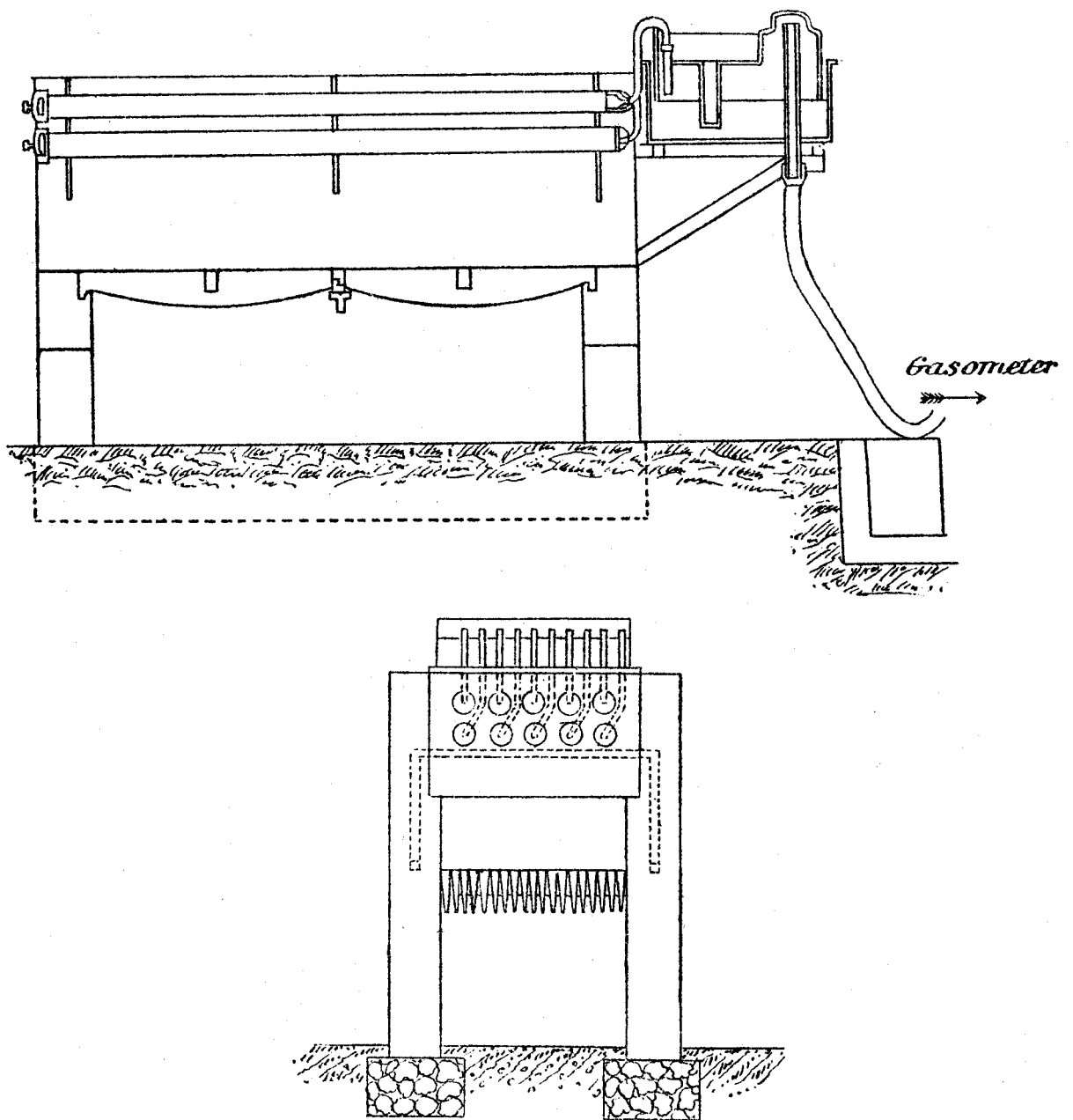
Figure 2.—Elevation and section of the apparatus used for generating marsh gas.
