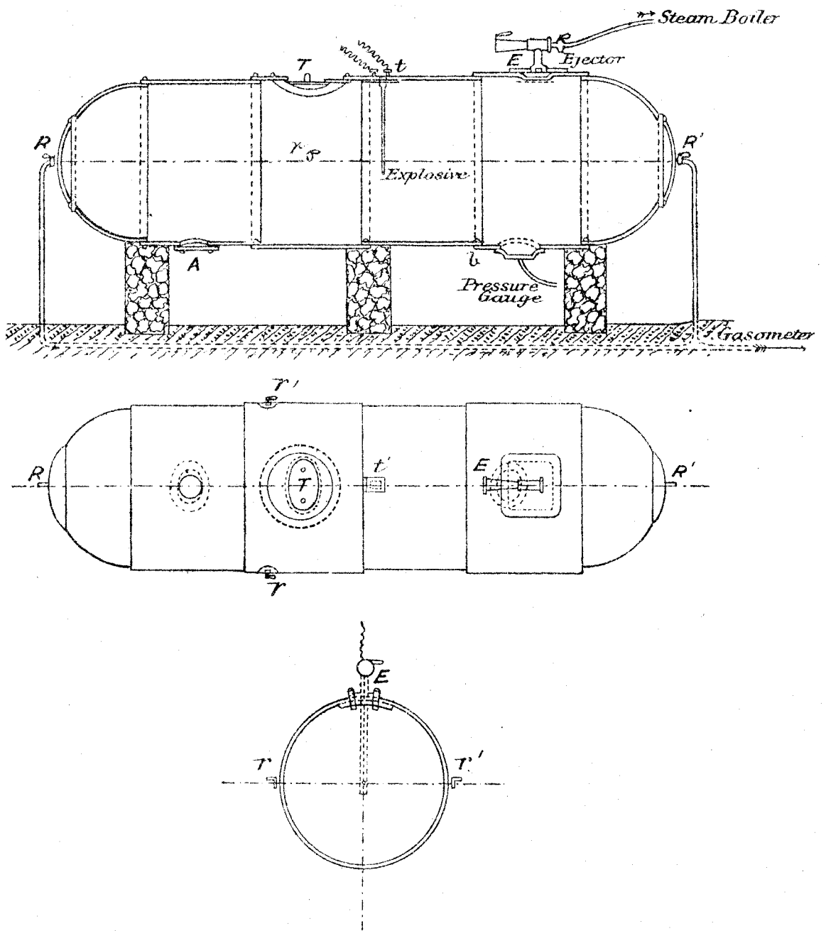
Figure 3.—Plan and sections of the boiler.
