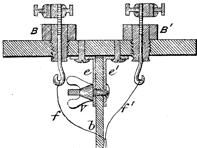
Figure 4.—Details of the attachment of the cartridge to the lid of the small hole of the boiler.
