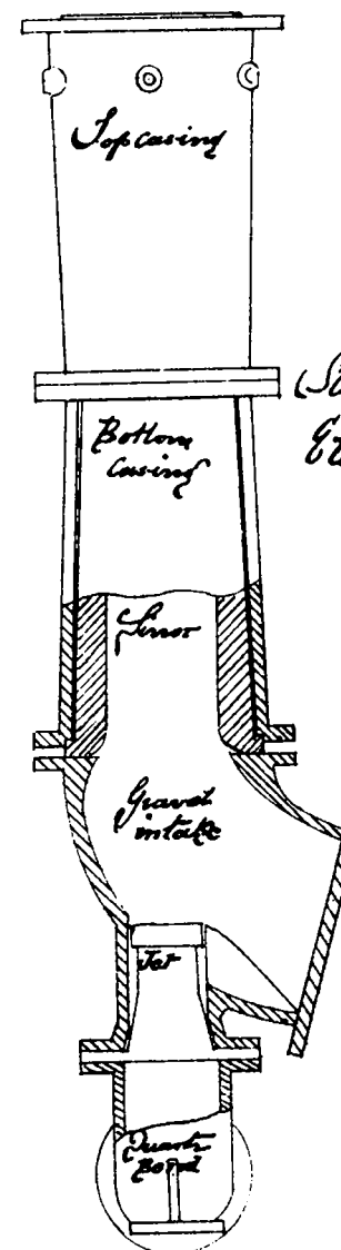
Side Elevation
