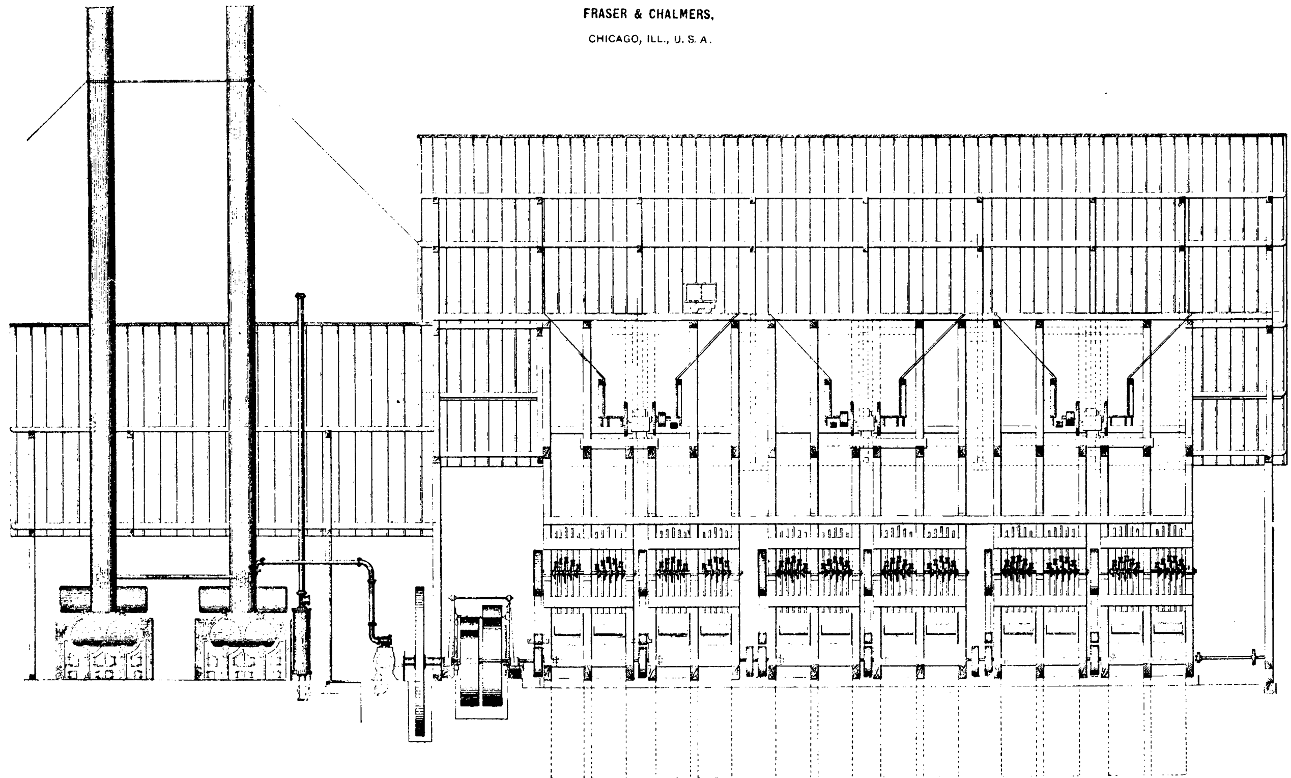
SECTIONS SHOWING CONSTRUCTION AND ARRANGEMENTS OF THE HIGHLAND MILL, LEADVILLE.
