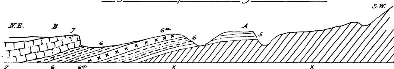
Fig 8. Sketch Section from Limestone South side of Maraewhenua River to Livingstone, showing position of the Auriferous Quartz Drifts relative to the Middle & Upper Parts of the Cretaceous-Tertiary Form. —
