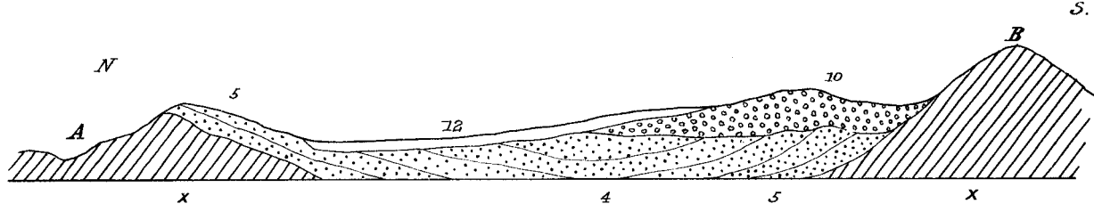
Fig 11. Sketch Section showing the position and relations of the Auriferous beds at Switzers to the underlying Quartz drifts, and of these to the Old Rocks. —————
