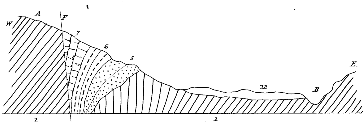
Fig 13. Sketch Section showing the manner of involvement of the Quartz-drifts on the slopes of Ben More, between Moke and Moonlight Creeks. Lake Wakatipu. —————
