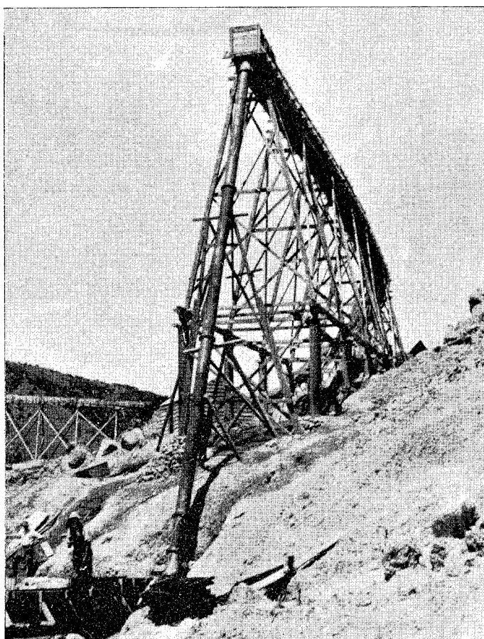
No. 1 Elevator.
