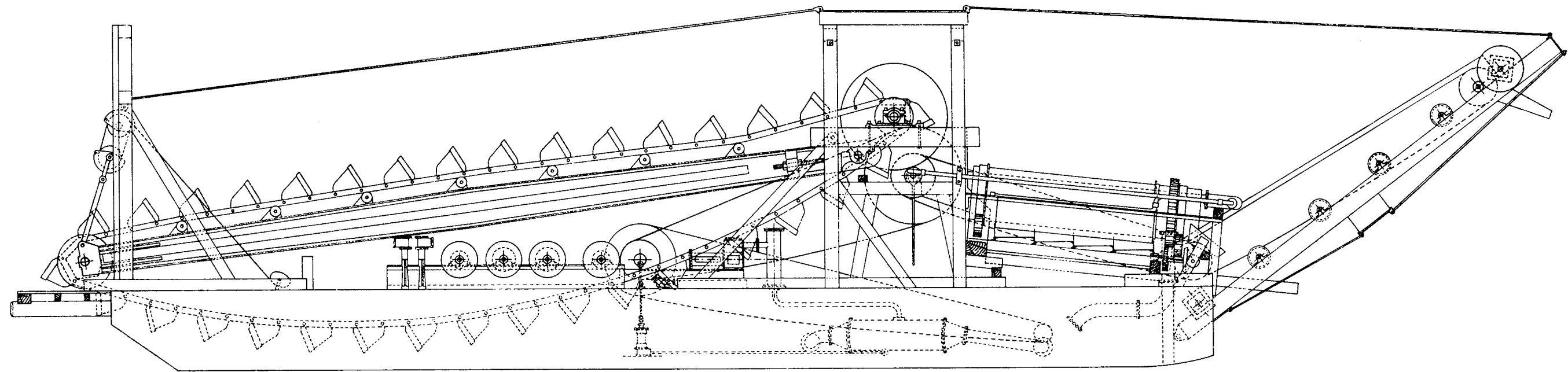
— SIDE ELEVATION (Boiler removed). —
