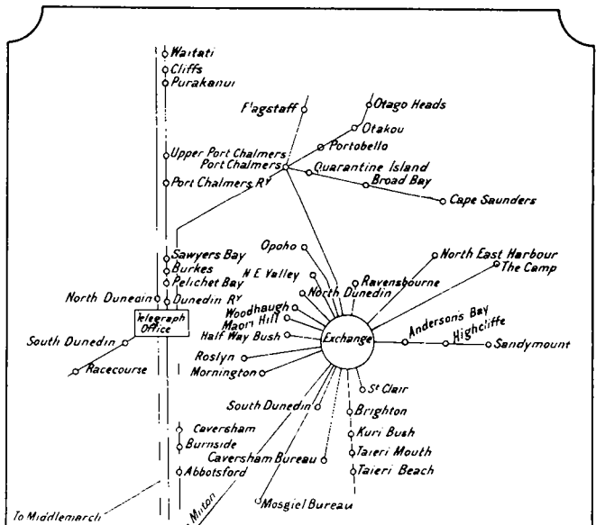
DUNEDIN DISTRICT Graphic Sketch of Connections
