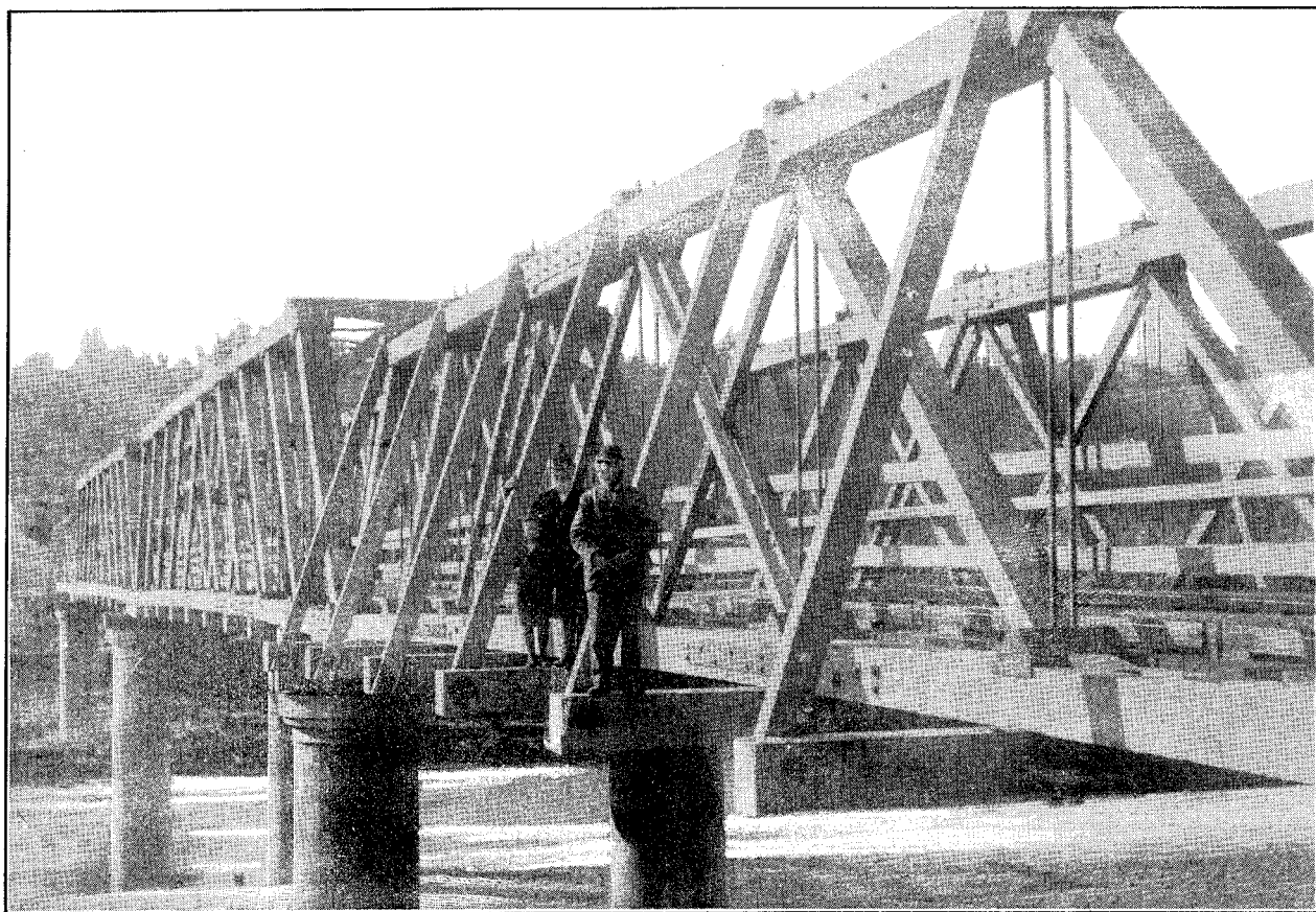
Vinegar Hill Bridge before Flood of 1897. Detail View from the South-west.
