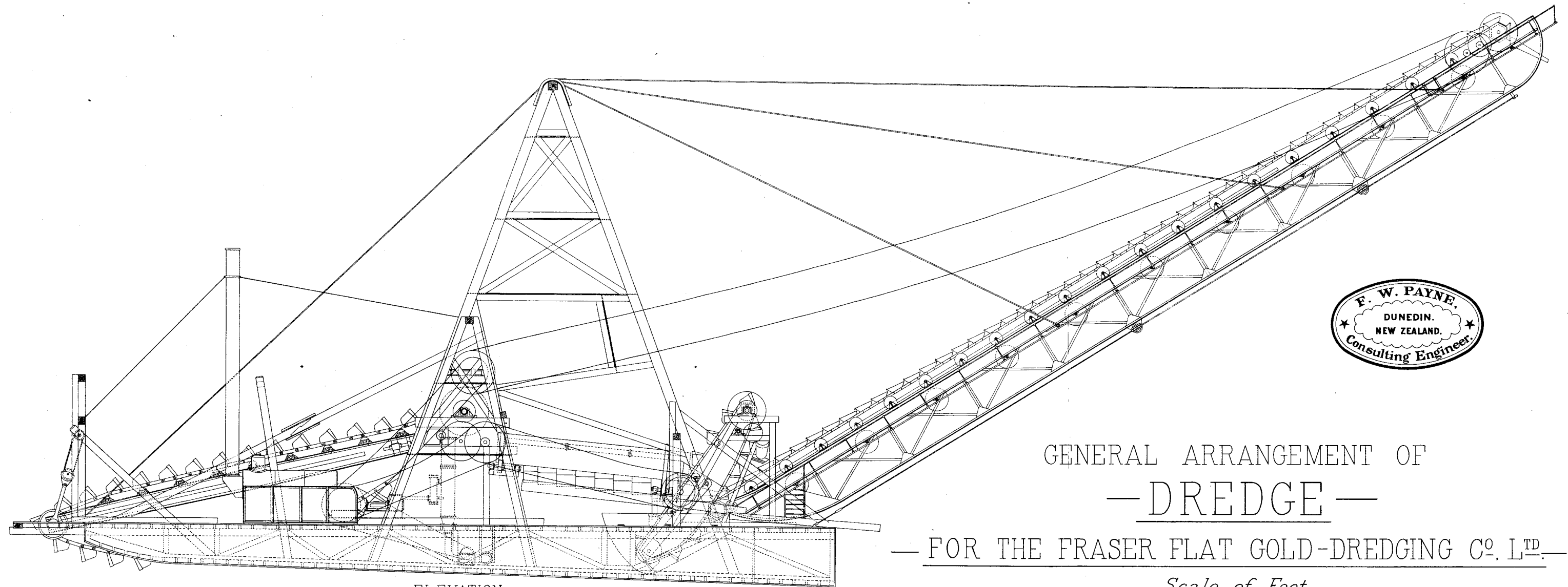
— ELEVATION. —
