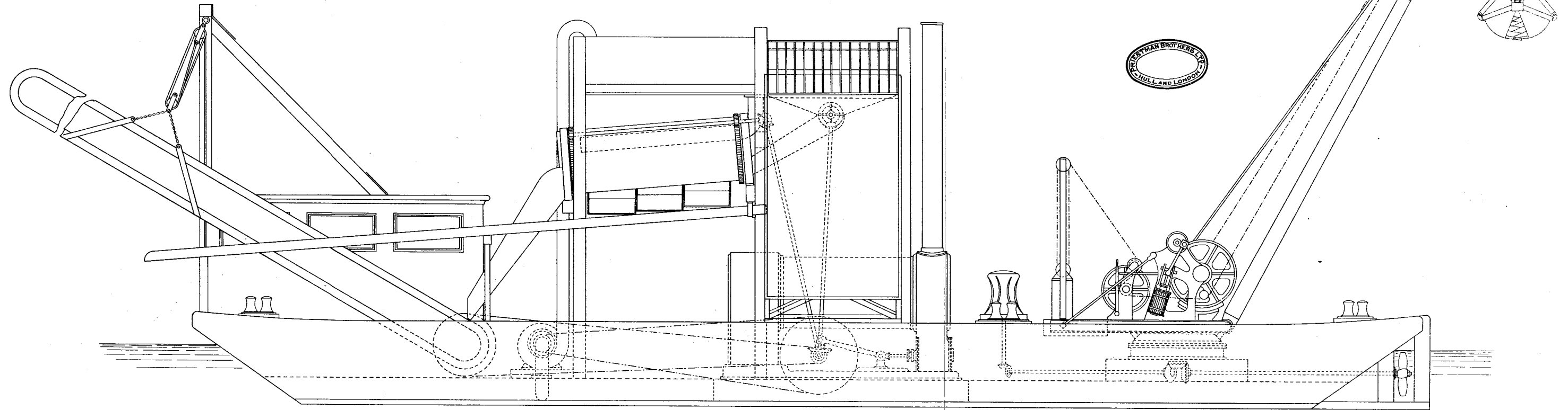
— ELEVATION. —
