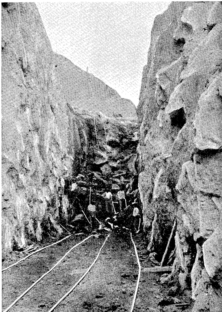
North Island Main Trunk Railway, Ohinemoa Section A Rhyolite Rock Cutting.
