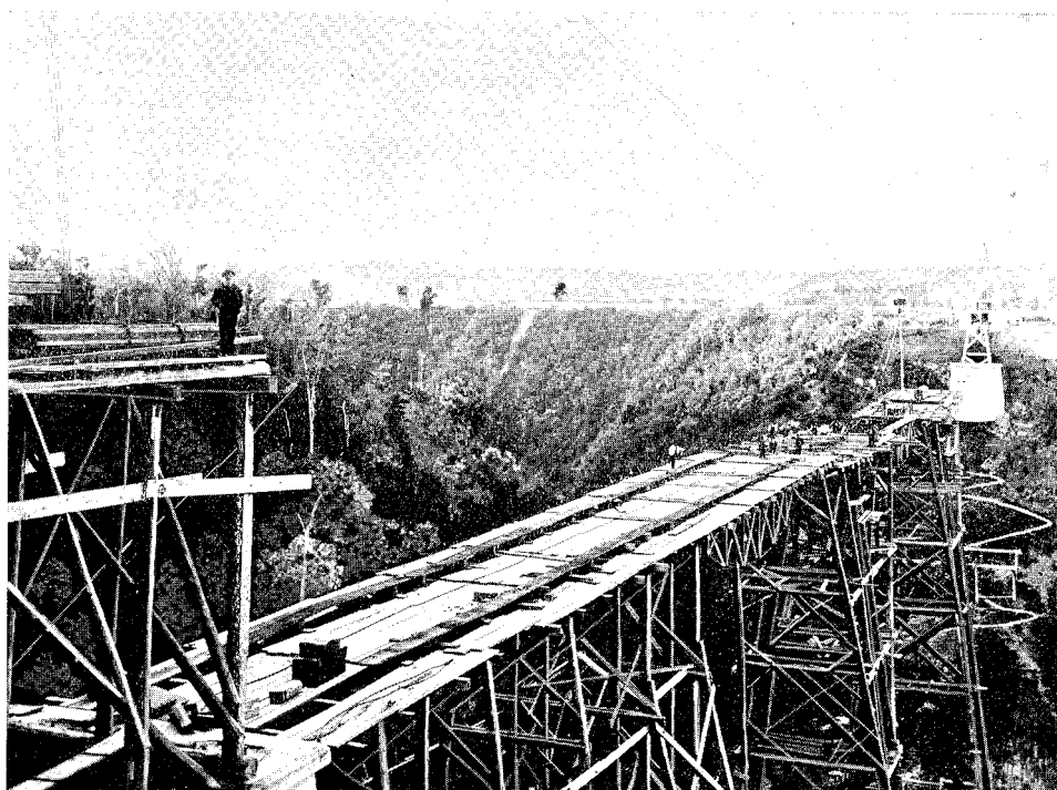
North Island Main Trunk Railway, Makohine Viaduct—Showing temporary Staging—View from Rail-level.
