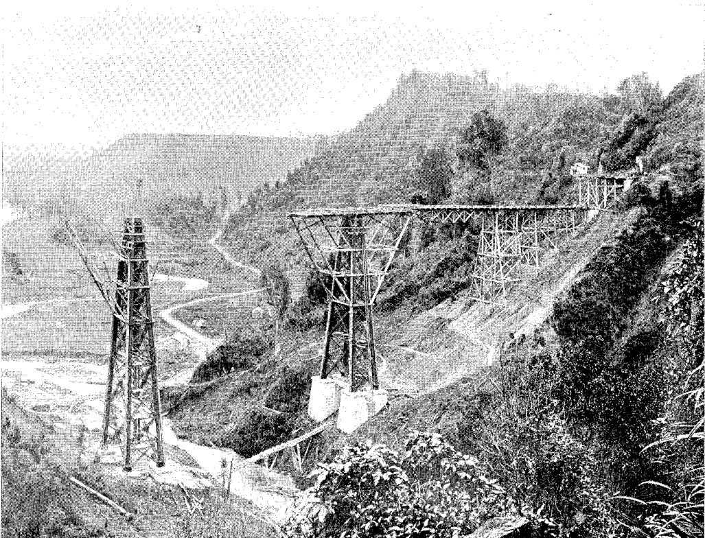
North Island Main Trunk Railway, Makohine Viaduct—Showing temporary Staging in course of Erection.
