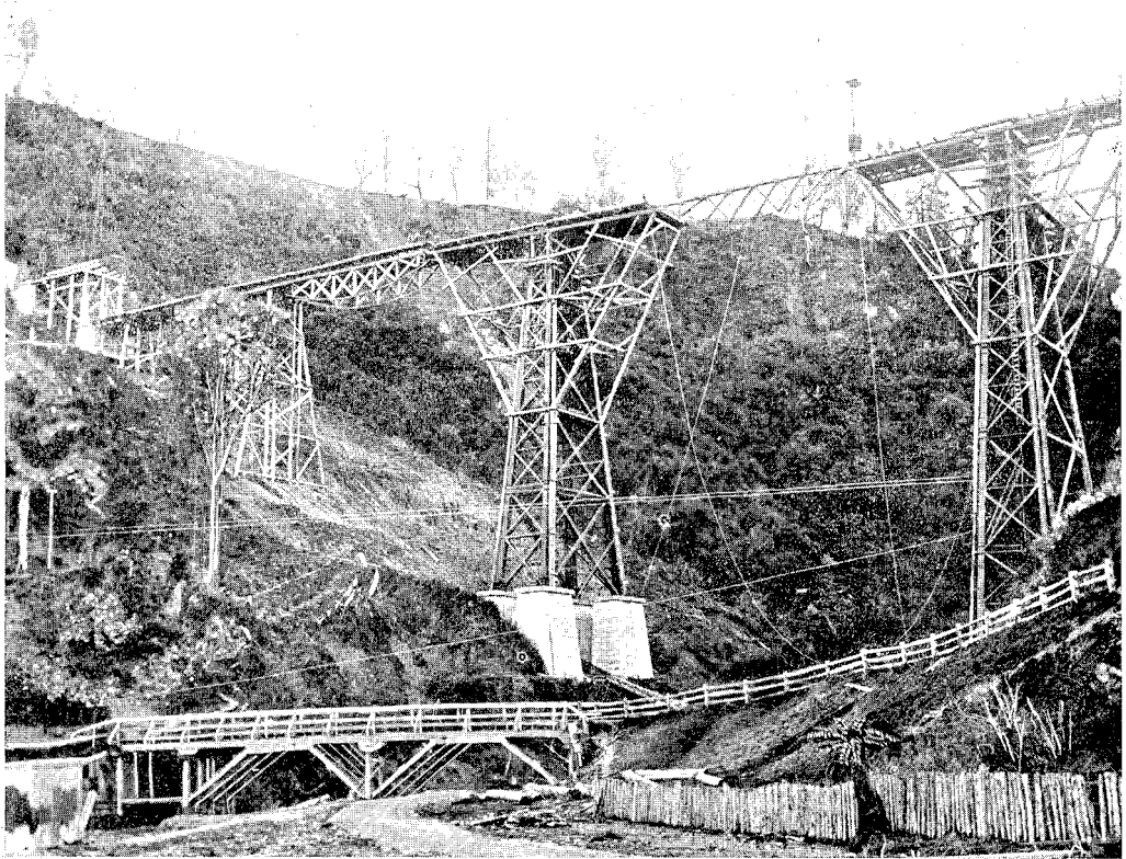
North Island Main Trunk Railway, Makohine Viaduct—Showing temporary Staging for Erection of Steel Superstructure.
