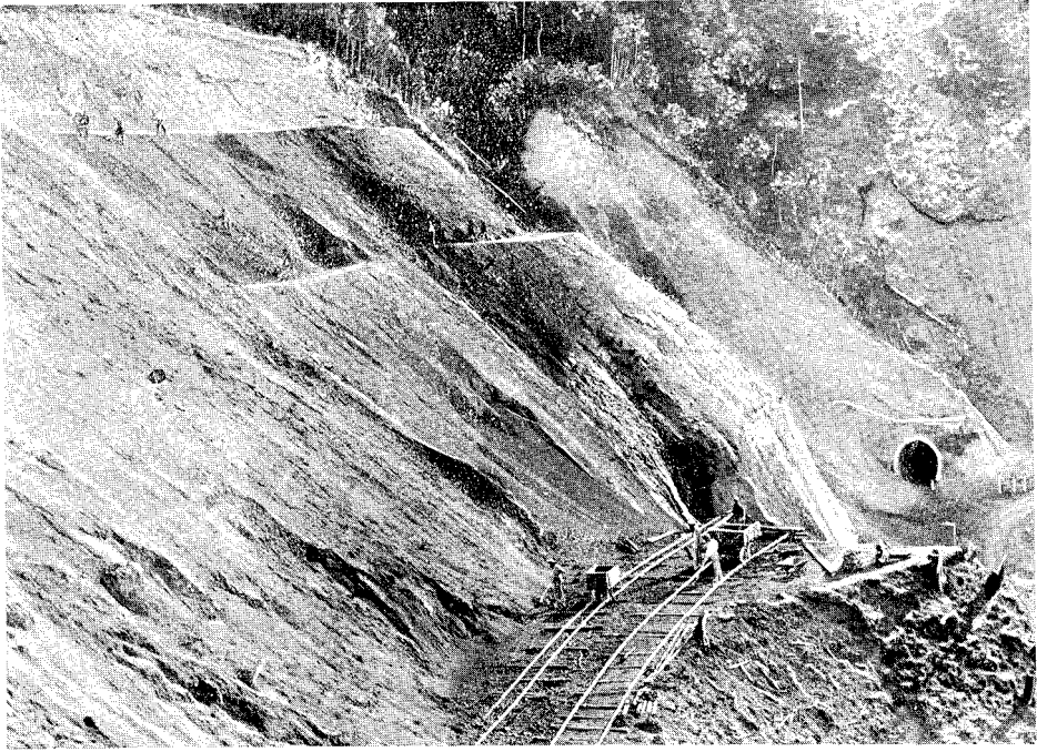
Midland Railway, Springfield End—Benching Batters near Tunnel No. 1.
