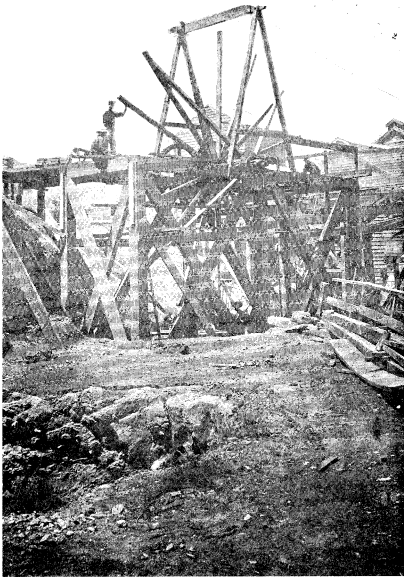
Erecting one of the large Elevating Wheels at the Waihi Gold-mining Company's 90-stamp Mill, Waihi.
