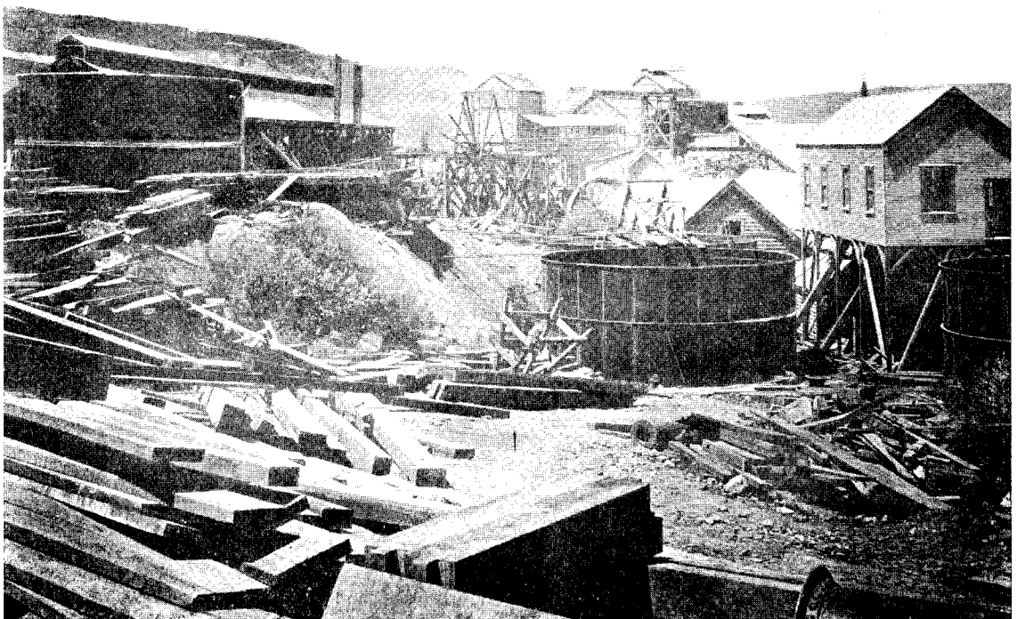
Erection of Elevating Wheels, Settlers, and Solution Tanks at the Waihi Gold-mining Company's 90-stamp Mill, Waihi. Face p. 93.] C.--3.
