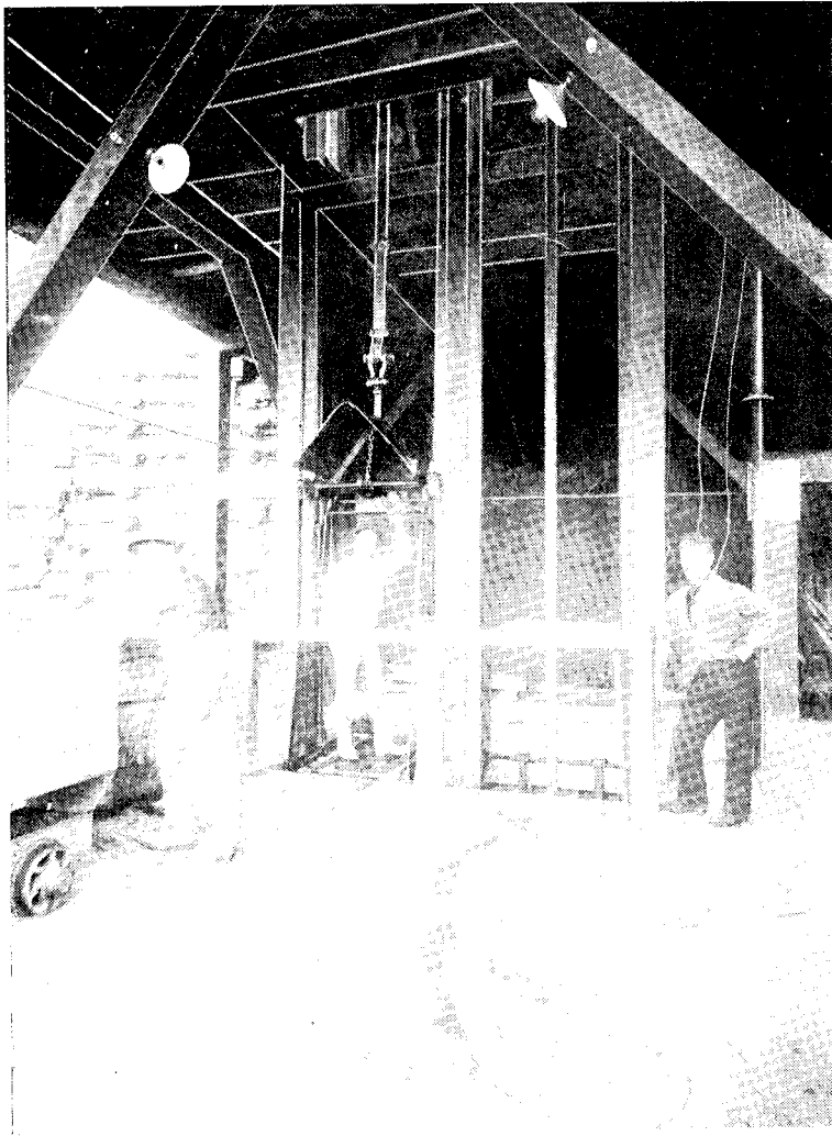
"B" Shaft-cage about to descend.
