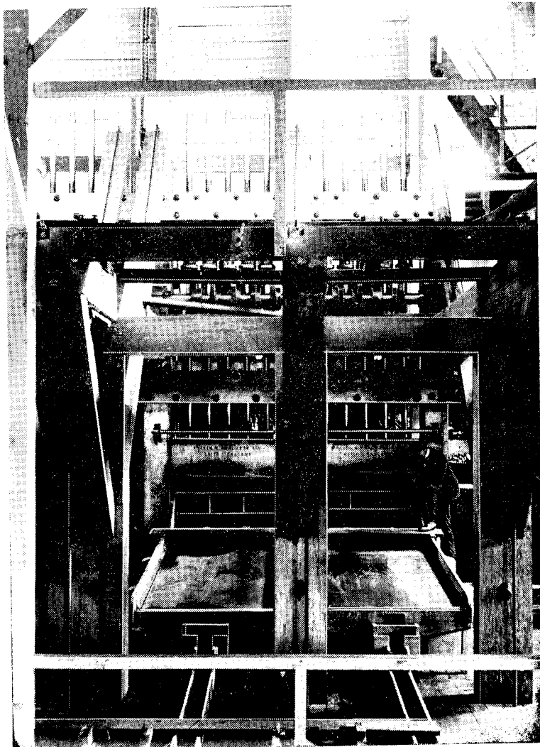
Face p. 105. Progress Mines 65-stamp Battery: View of Ten Stamps O.—3.
