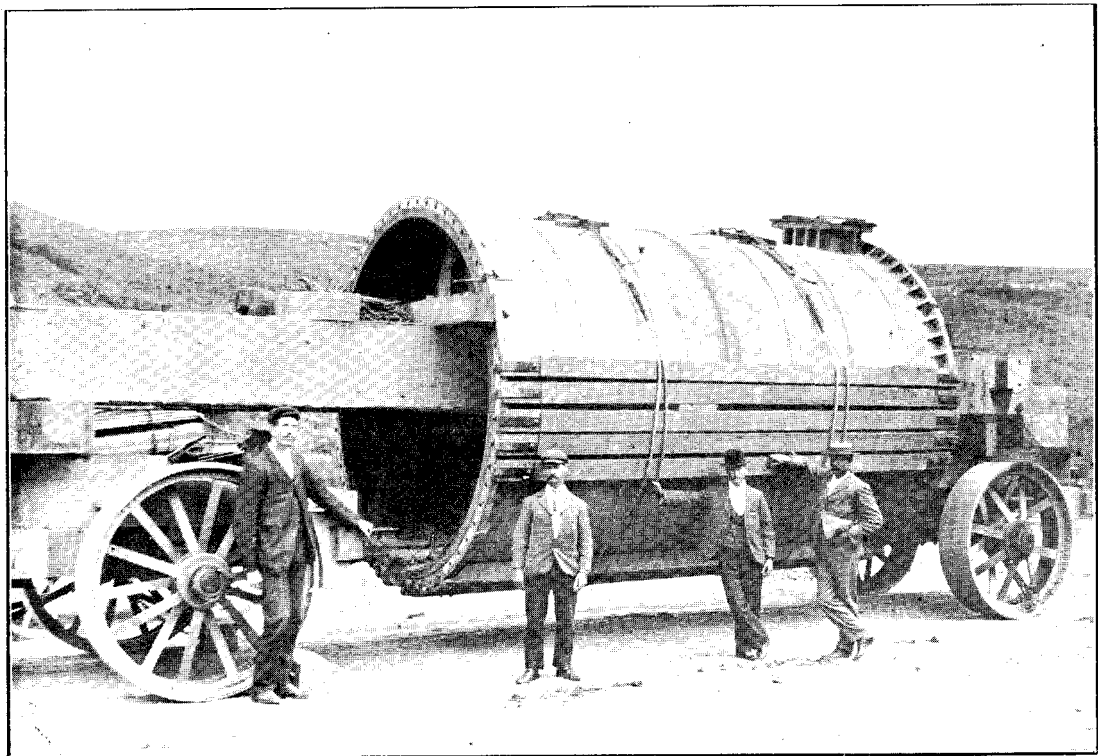
LOW-PRESSURE CYLINDER OF NEW PUMPING ENGINE (WAIHI MINE) IN TRANSIT. DIAMETER 110", STROKE 12' 0".
