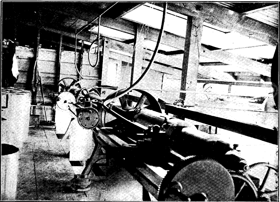
ZINC-CUTTING MACHINES, WAIKINO BATTERY, WAIHI GOLD-MINING COMPANY.
