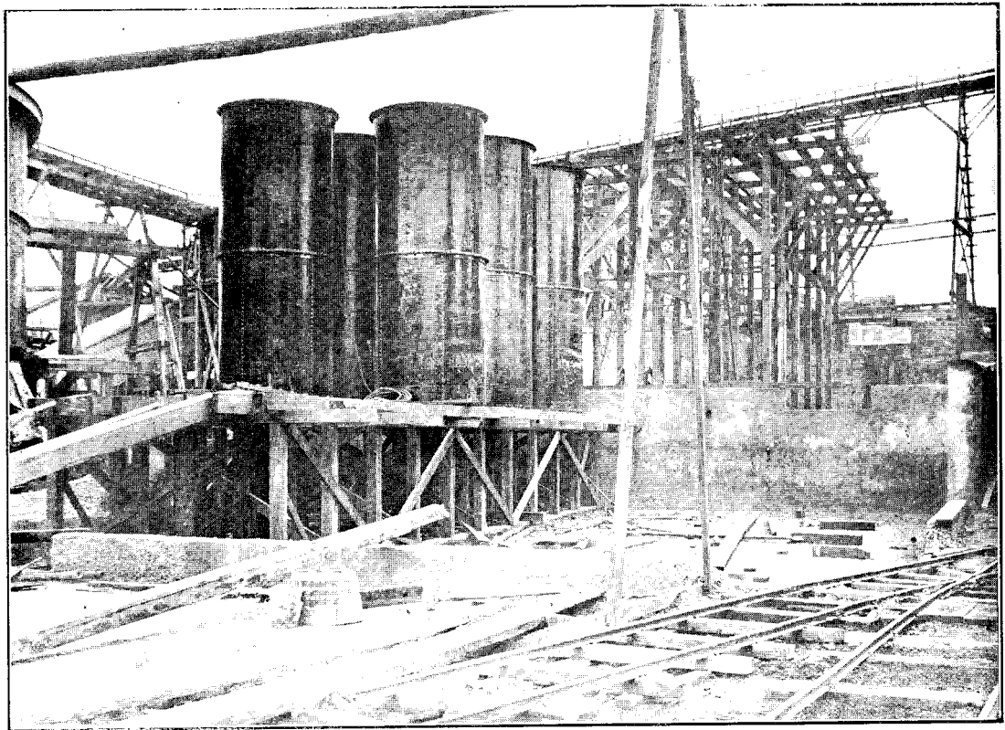
CONCENTRATES TREATMENT PLANT, WAIKINO BATTERY, IN COURSE OF ERECTION (WAIHI GOLD-MINING COMPANY).
