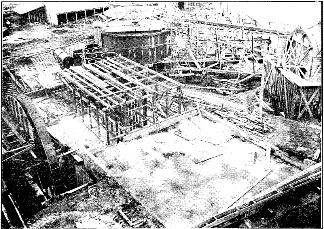
CONCENTRATES TREATMENT PLANT, WAIKINO BATTERY, IN COURSE OF ERECTION (WAIHI GOLD-MINING COMPANY).
