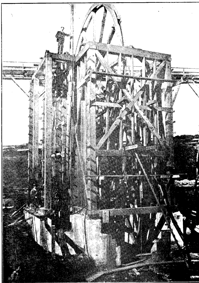
GROUP OF FOUR ELEVATOR WHEELS, DOUBLE LIFT, WAIKINO BATTERY, WAHI GOLD-MINING COMPANY.
