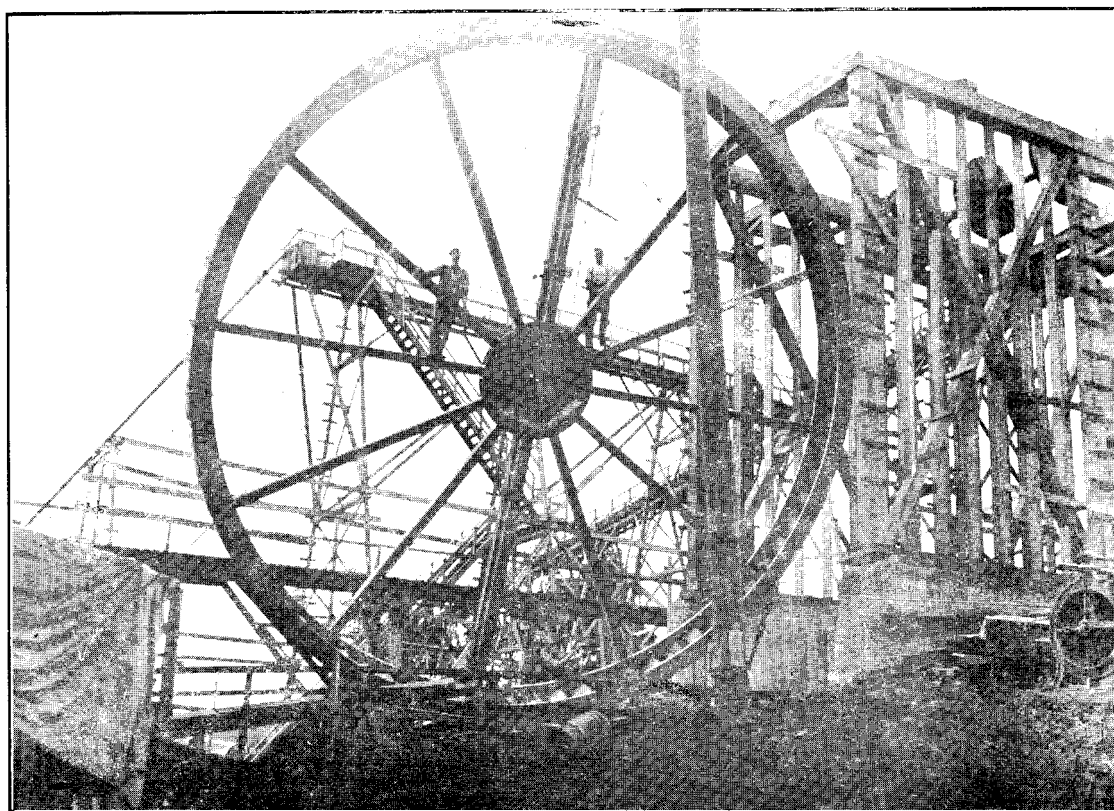
ELEVATOR WHEEL, WAIKINO BATTERY, BEING PLACED IN POSITION, WAHI GOLD-MINING COMPANY. DIAMETER, 35 FT. ; BUCKETS, 2' 0" WIDE.
