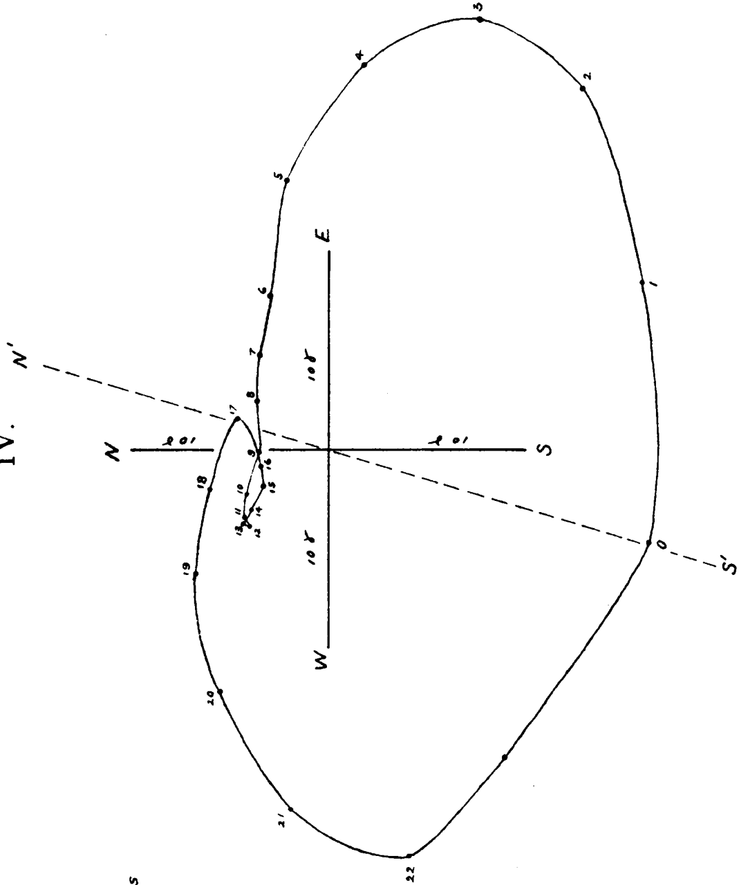
Vector Diagram of Horizontal Disturbing Forces for Greenwich Hours Year 1902, 3, 4.
