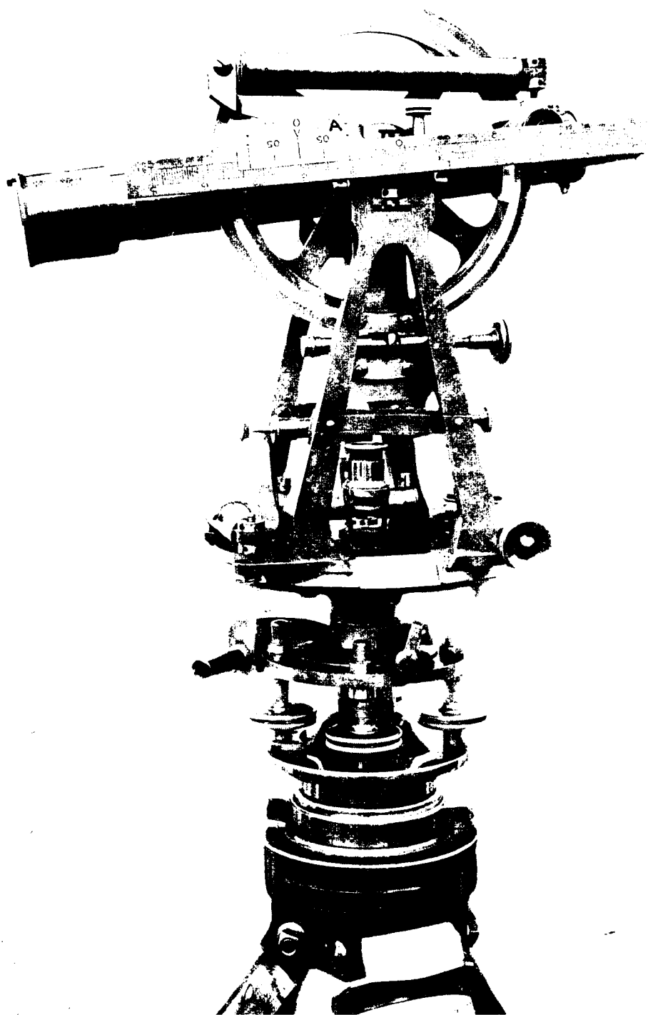
FIVE INCH TROUGHTON AND SIMMS TRANSIT, PHOTOGRAPH TAKEN AT A 90° DIVISION TO 20 SECONDS, WITH CHAINING SCALE IN POSITION.
