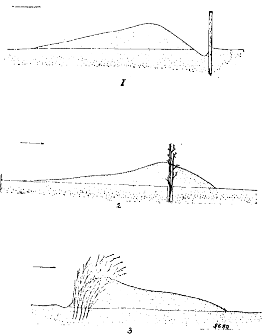
No. 9. (1.) EFFECT OF A SOLID OBSTACLE. (2.) EFFECT OF AN INFLEXIBLE OPEN OBSTACLE. (3.) EFFECT OF A FLEXIBLE OPEN OBSTACLE, SUCH AS A BUNCH OF MARRAM GRASS. (AFTER GERHARDT.)
