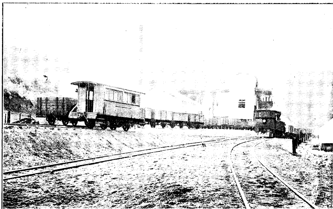
COAL SCREENING PLANT AND RAILWAY-SIDINGS. THE WAIPA RAILWAY AND COLLIERY COMPANY, GLEN MASSEY (WAIKATO COALFIELD).
