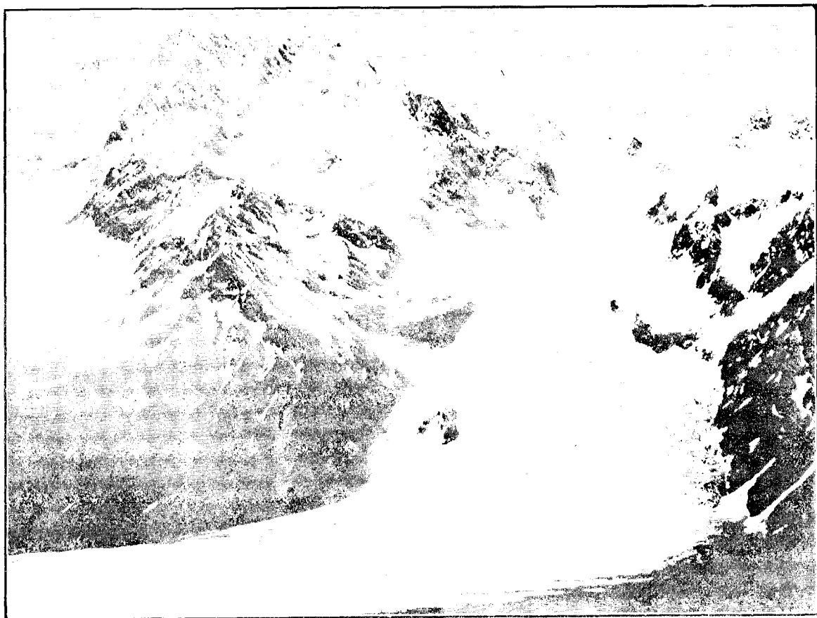
Hochstetter Ice Falls.
