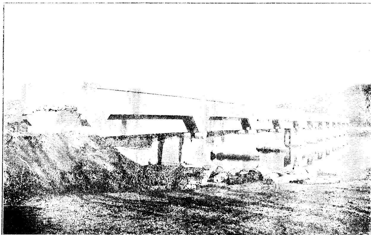
ROAD BRIDGE OVER WAOA RIVER, TAURANGA COUNTY Elevation of 141 ft. Total Length, 196 ft. Width between Wheel guards, 19 ft. Piers, Abutments, and Superstructure of Reinforced Concrete.
