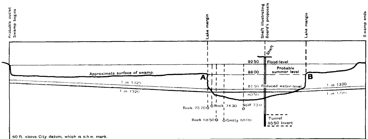
Longitudinal sketch of lake and swamp. Horizontal scale: 25 chains to an inch. Vertical scale: 25 feet to an inch.
