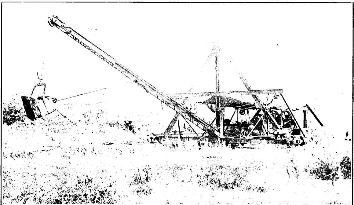
WALKING LAND DIPPER (12 CUBIC YARDS). (One purchased for New Zealand Government.)
