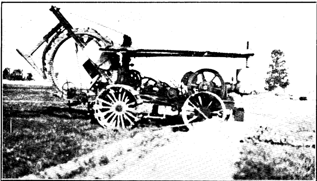
A TILE-DITCHER.
