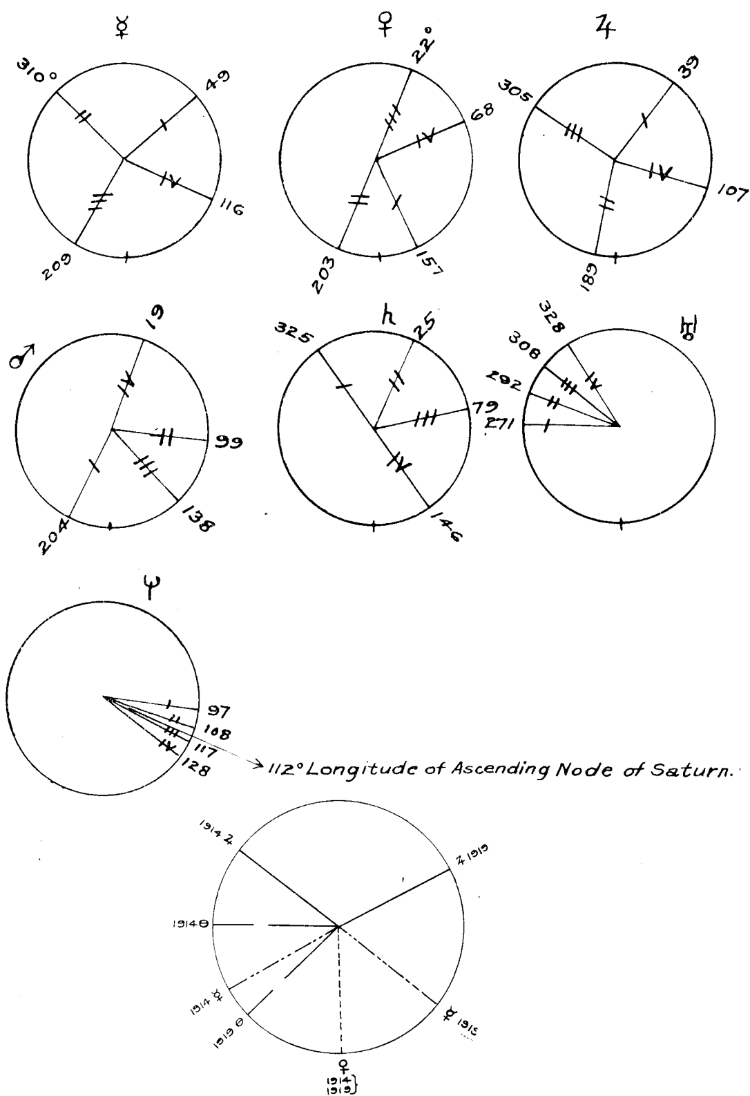
DIAGRAMS REFERRING TO PLANETARY-SOLAR EFFECT ON HORIZONTAL MAGNETIC FORCE.
