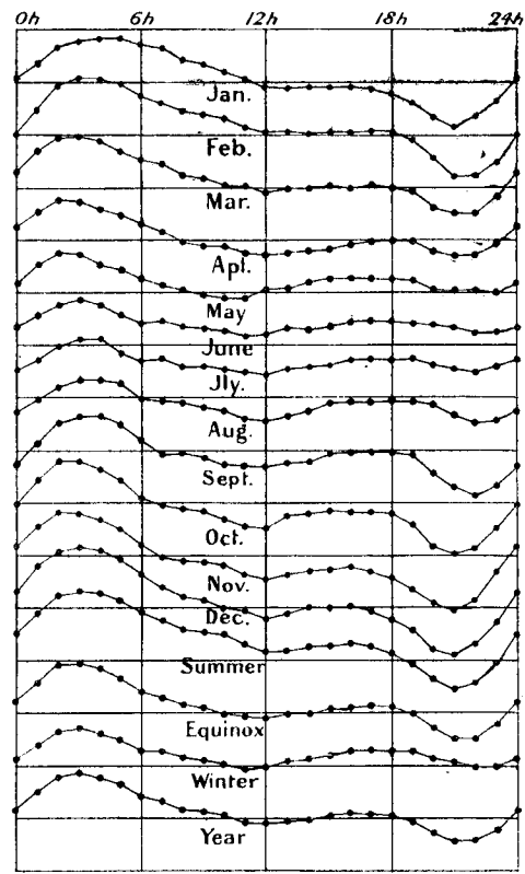
MEAN DIURNAL DECLINATION FOR 1921
