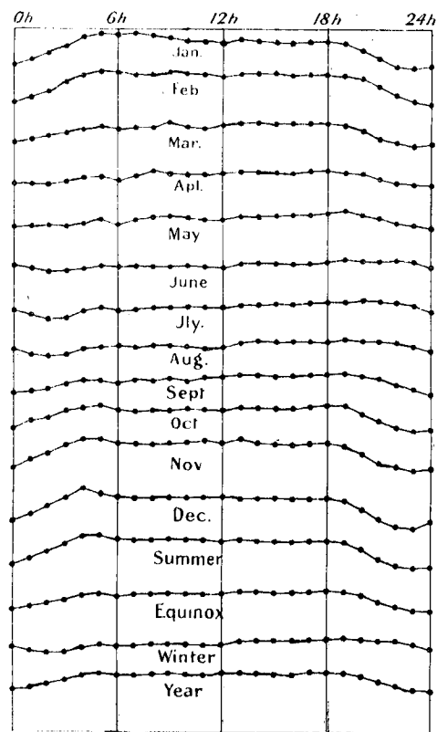
MEAN DIURNAL HORIZONTAL FORCE, 1921.
