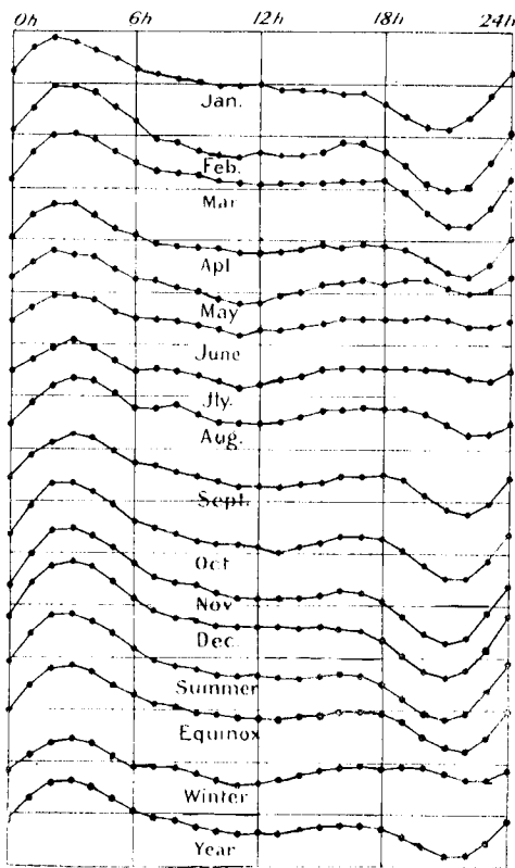
MEAN DIURNAL DECLINATION FOR 1907.
