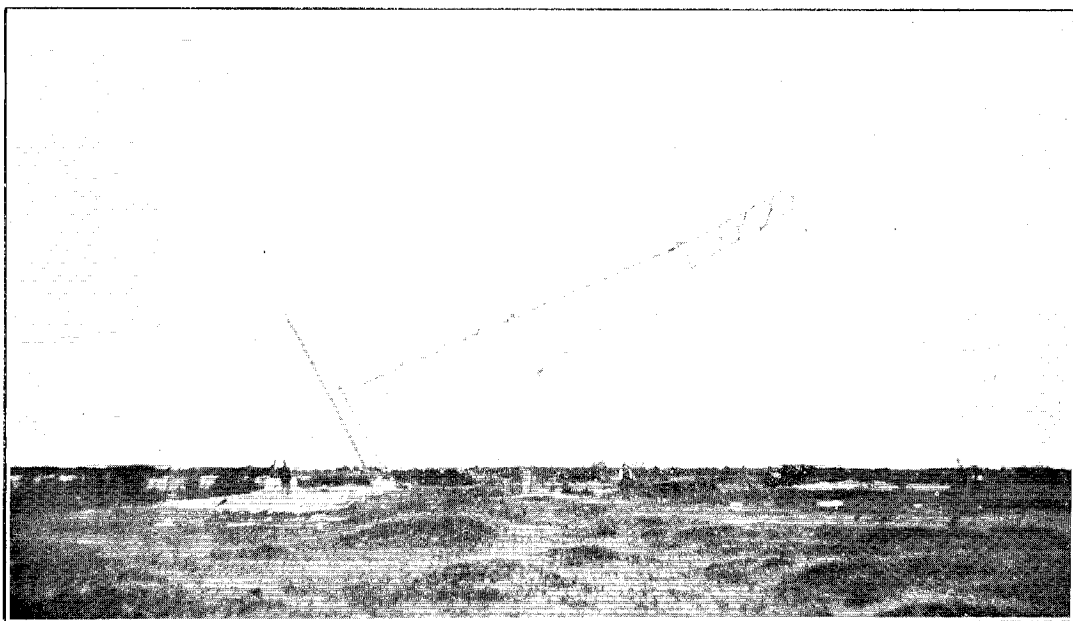
LAKE COLERIDGE HYDRO-ELECTRIC-POWER PLANT: METHOD OF ERECTING TRANSMISSION-LINE TOWERS.
