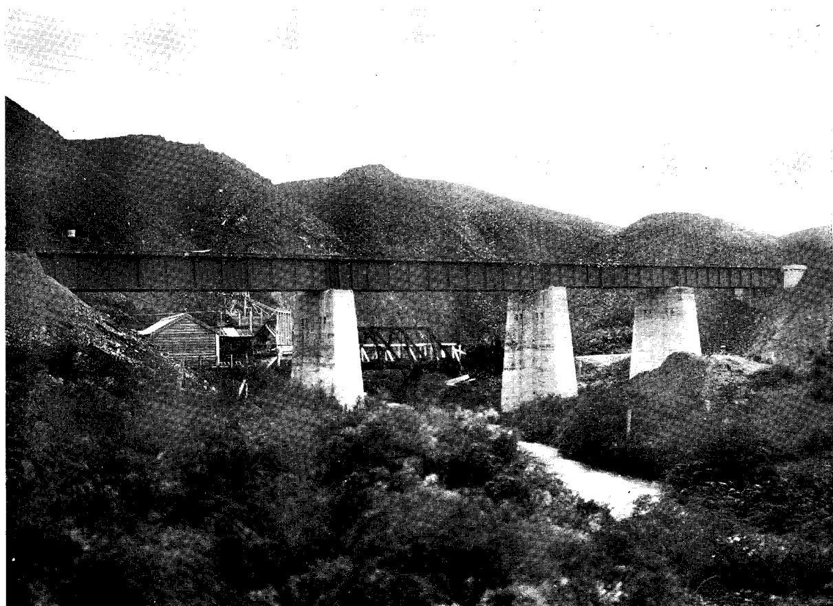
EAST COAST MAIN TRUNK RAILWAY, ATHENREE SECTION. Bridge at 70 m. 23 ch. (Quarry in background.)
