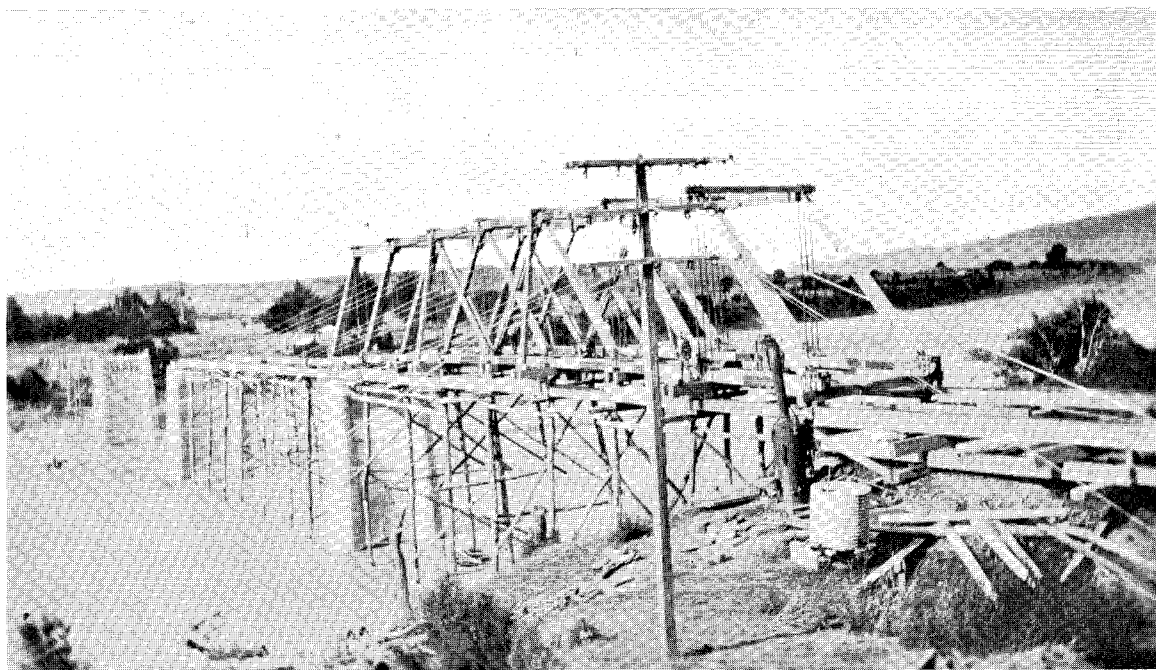
ROKOKAUTUKU BRIDGE UNDER CONSTRUCTION. (Span erected on shore and launched out on skidways.)
