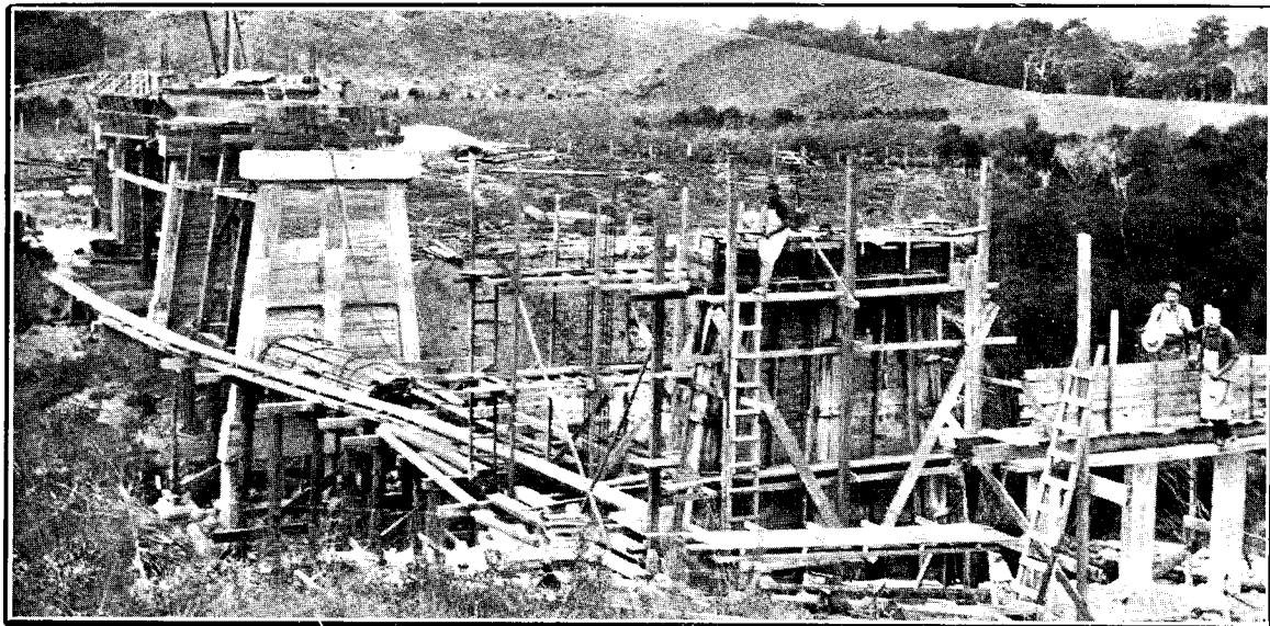
WAIWERA-MANGAWAI MAIN HIGHWAY: HOTOE RIVER BRIDGE UNDER CONSTRUCTION.
