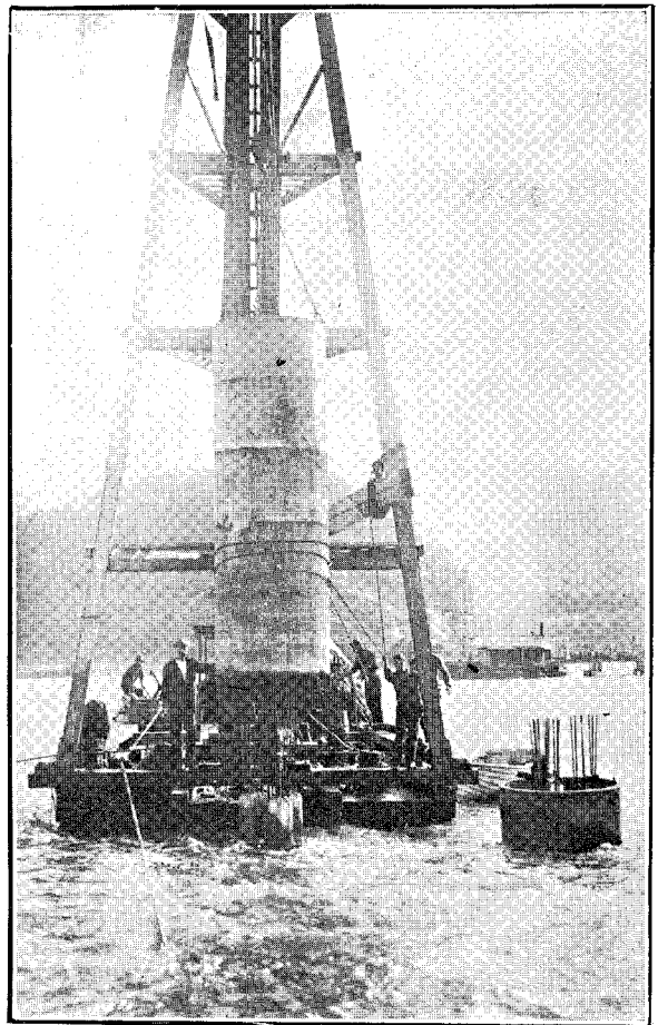
Lowering 5 ft. Diameter Concrete Casings over Piles.
