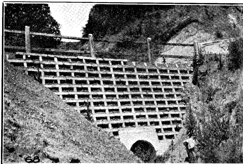
PETANE-TAUPO MAIN HIGHWAY: CULVERT AND CONCRETE CRIB RETAINING-WALL.
