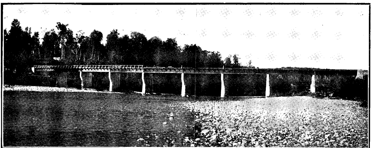
WESTPORT-NELSON MAIN HIGHWAY : INANGAHUA JUNCTION BRIDGE NEARING COMPLETION. WIDE PIERS PROVIDED FOR FUTURE RAILWAY-BRIDGE.
