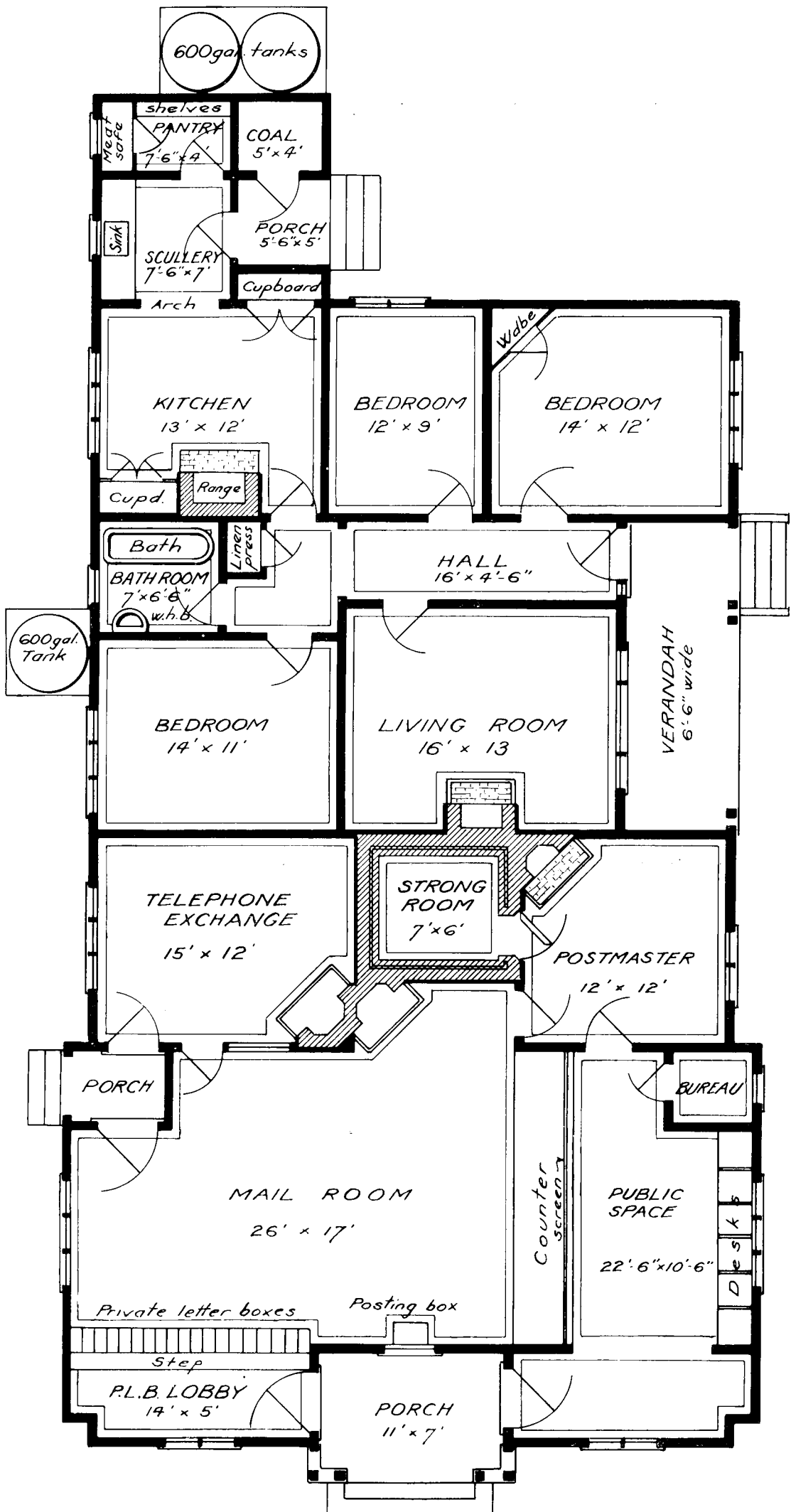
PLAN OF TUATAPERE POST-OFFICE BUILDING A TYPE OF COUNTRY POST-OFFICE WITH QUARTERS.
