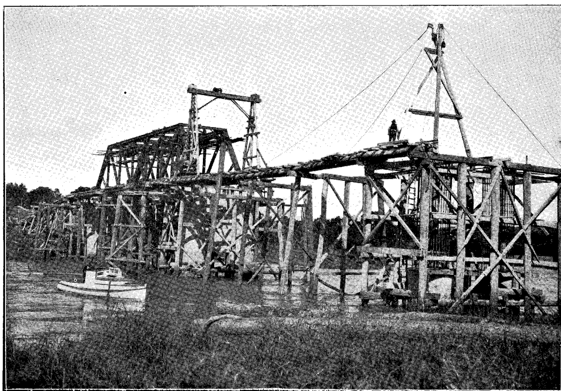
NORTHERN WAIROA BRIDGE UNDER CONSTRUCTION.
