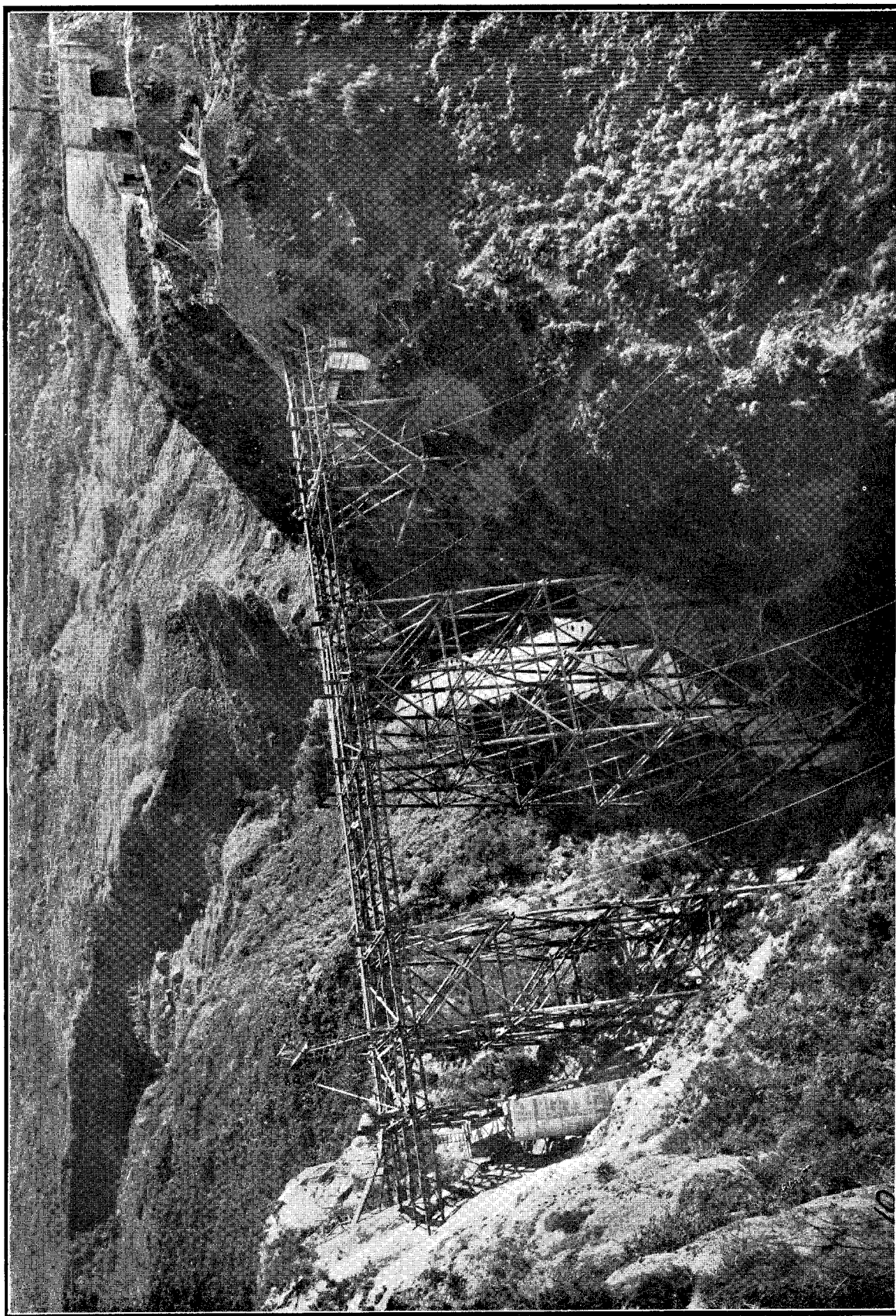
WAIKOAU VIADUCT UNDER CONSTRUCTION. Trestling for erection of main 250 ft. span. NAPIER-WAIROA RAILWAY.
