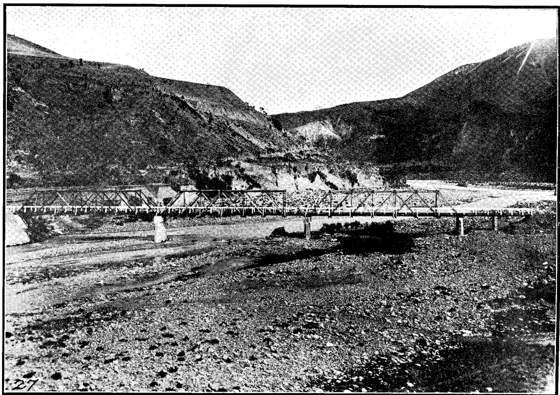
AWATERE RIVER ROAD-BRIDGE : ACCESS TO MEDWAY. Three 110 ft. spans and three 25 ft. spans.
